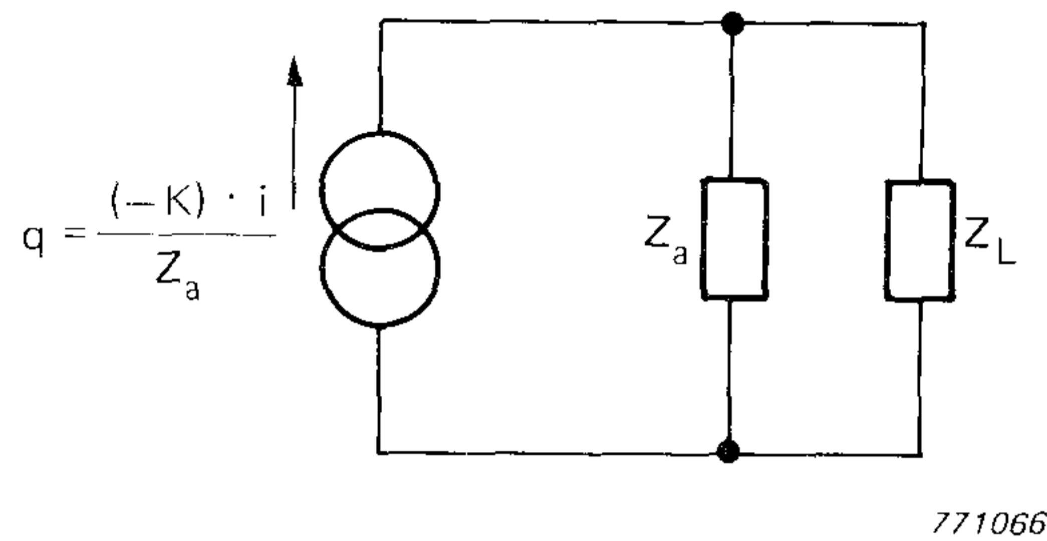
Fig.3. Simplified Equivalent Circuit of Calibrator 4221
