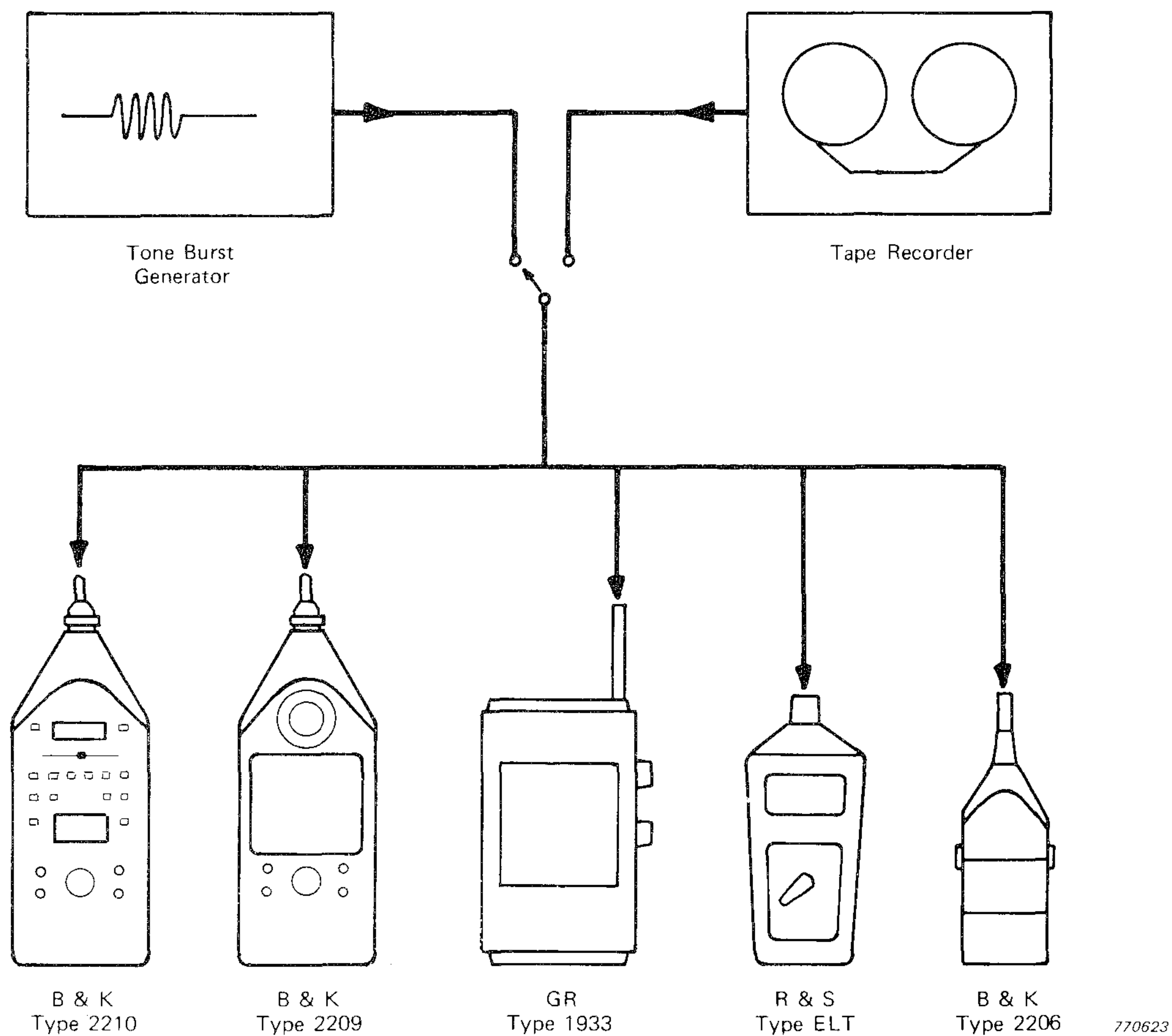
Fig.8. Set-up for measuring the impulse response of Sound Level Meters of different Types and manufacture
