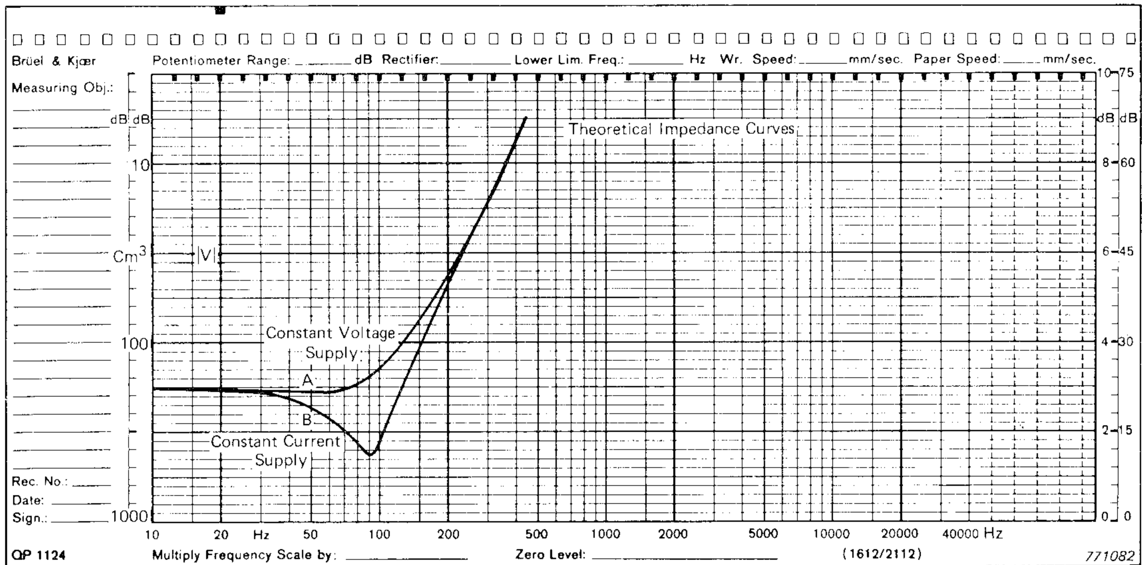
Fig.A1. Theoretical Impedance Curves of Calibrator 4221
