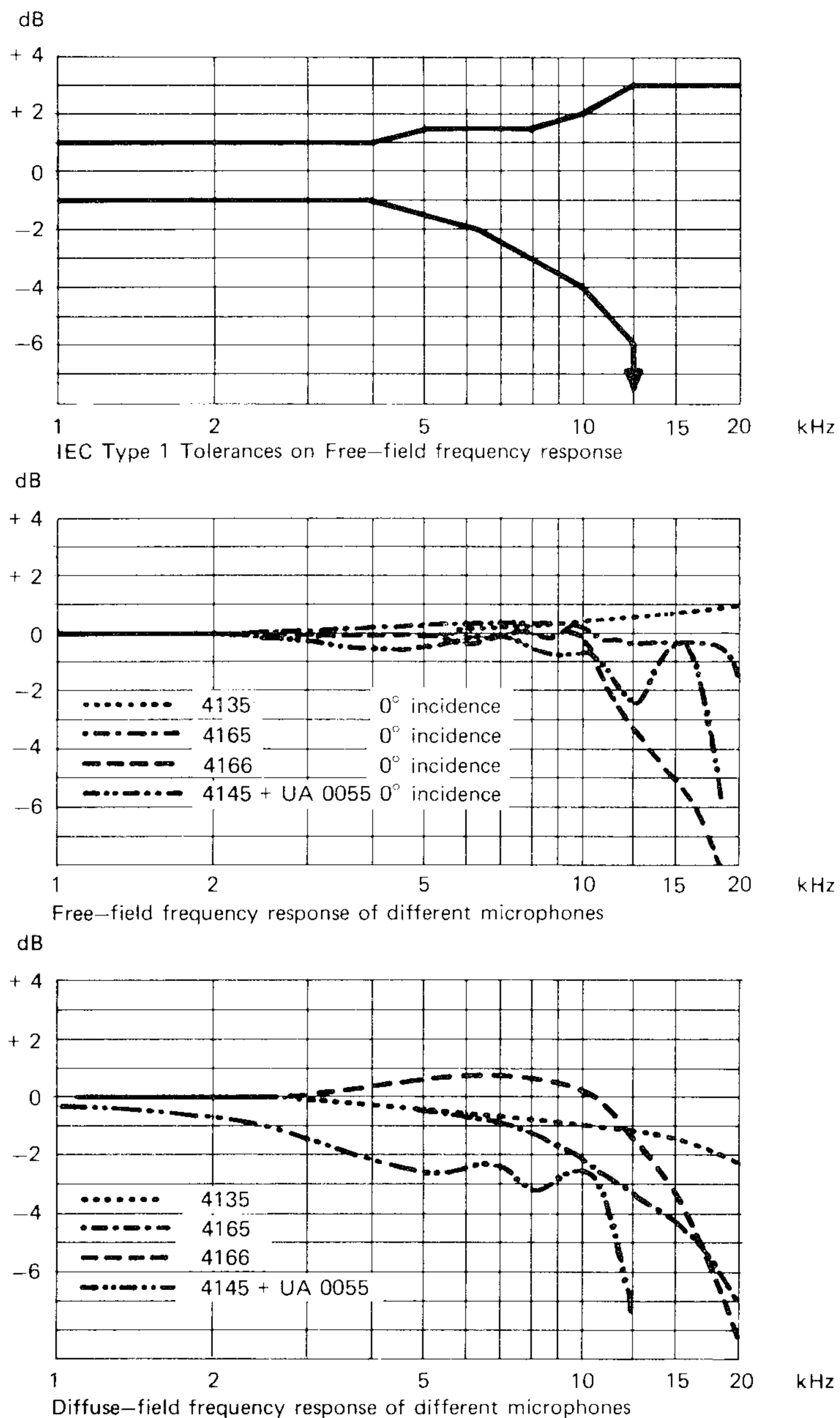
Fig.2. Comparison between IEC Type 1 Tolerances for free-field frequency response and the free-field response of microphones of different sizes
