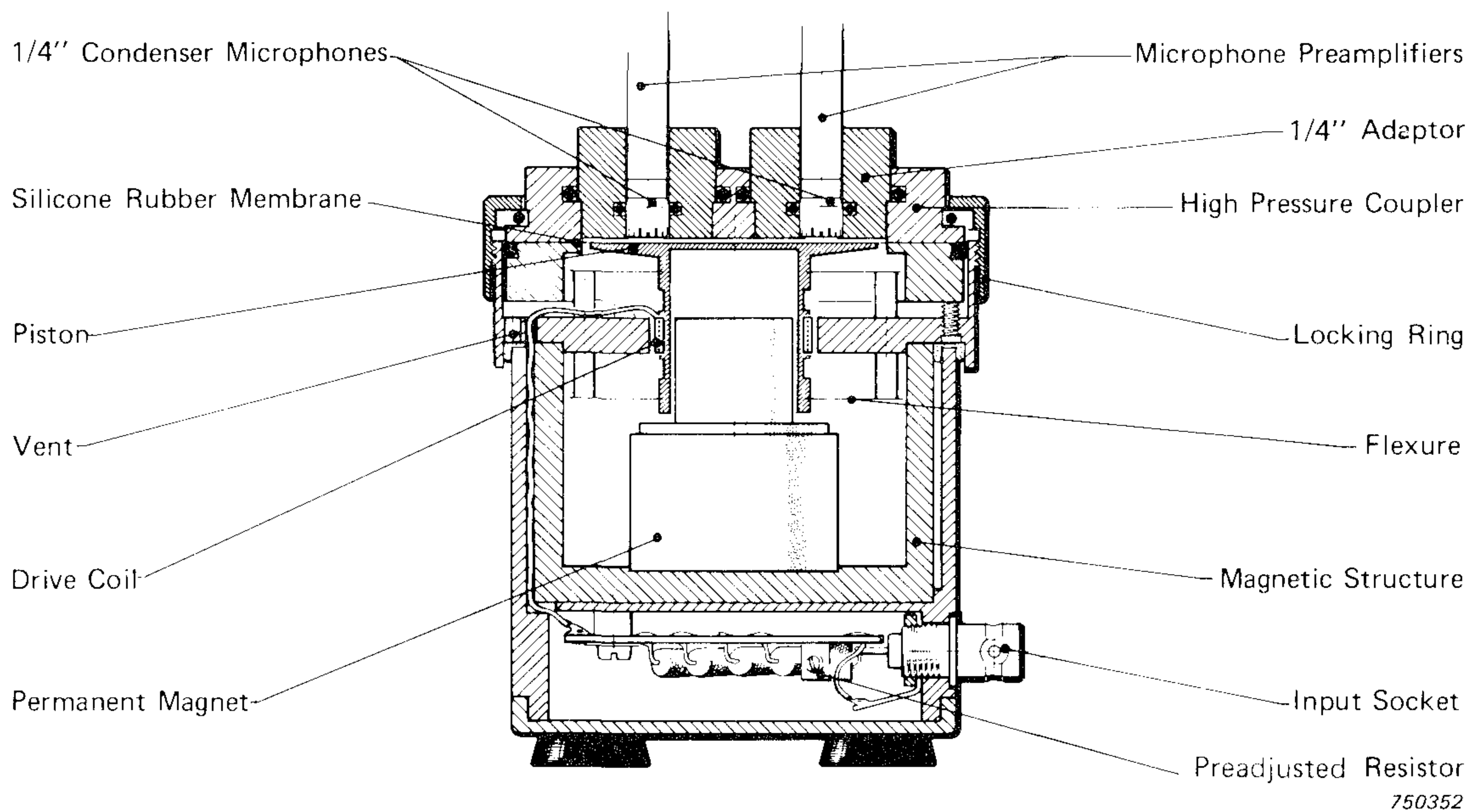
Fig.1. Cross Sectional View of Calibrator 4221
