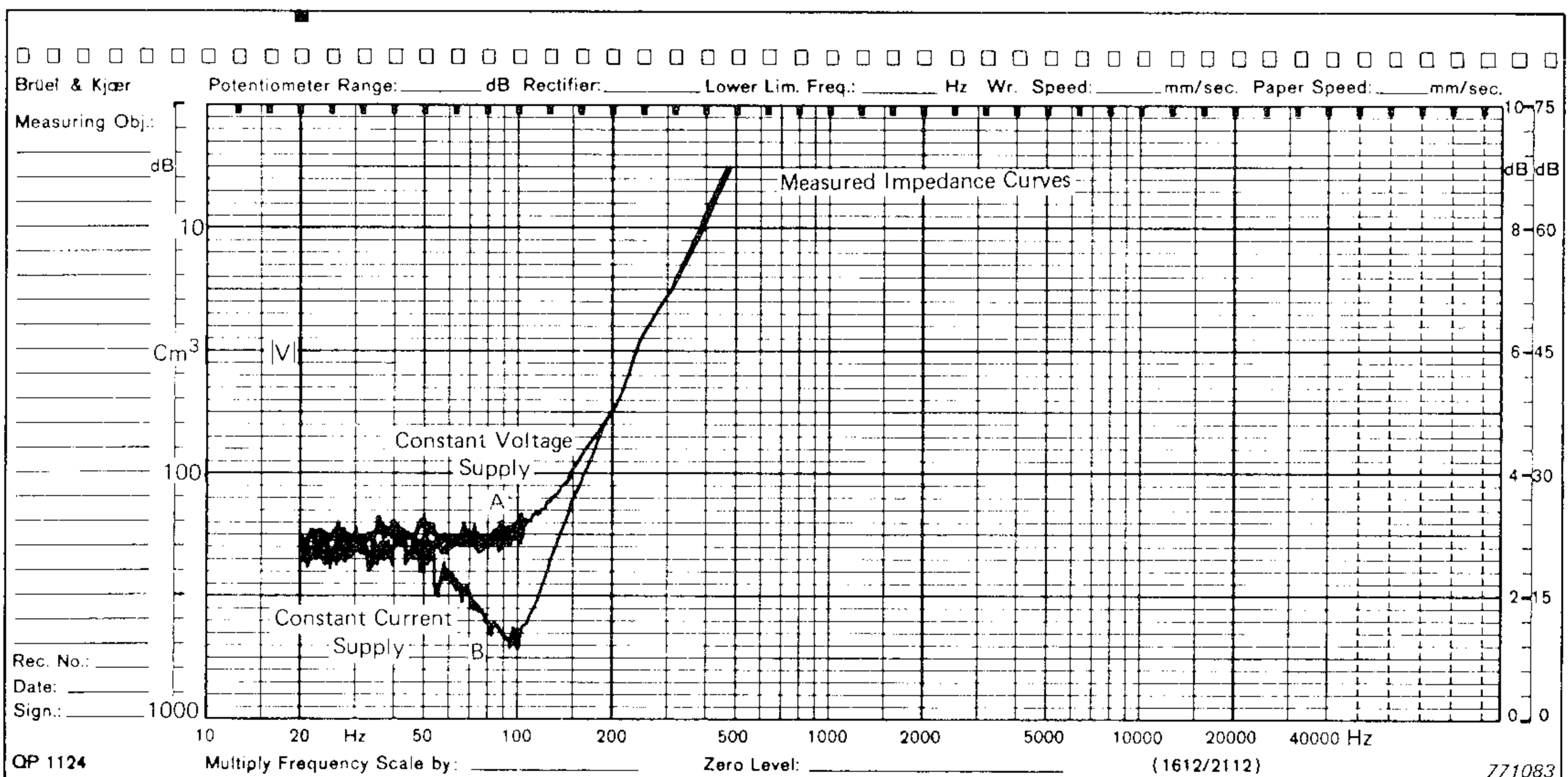
Fig.A2. Measured Impedance Curves of Calibrator 4221
