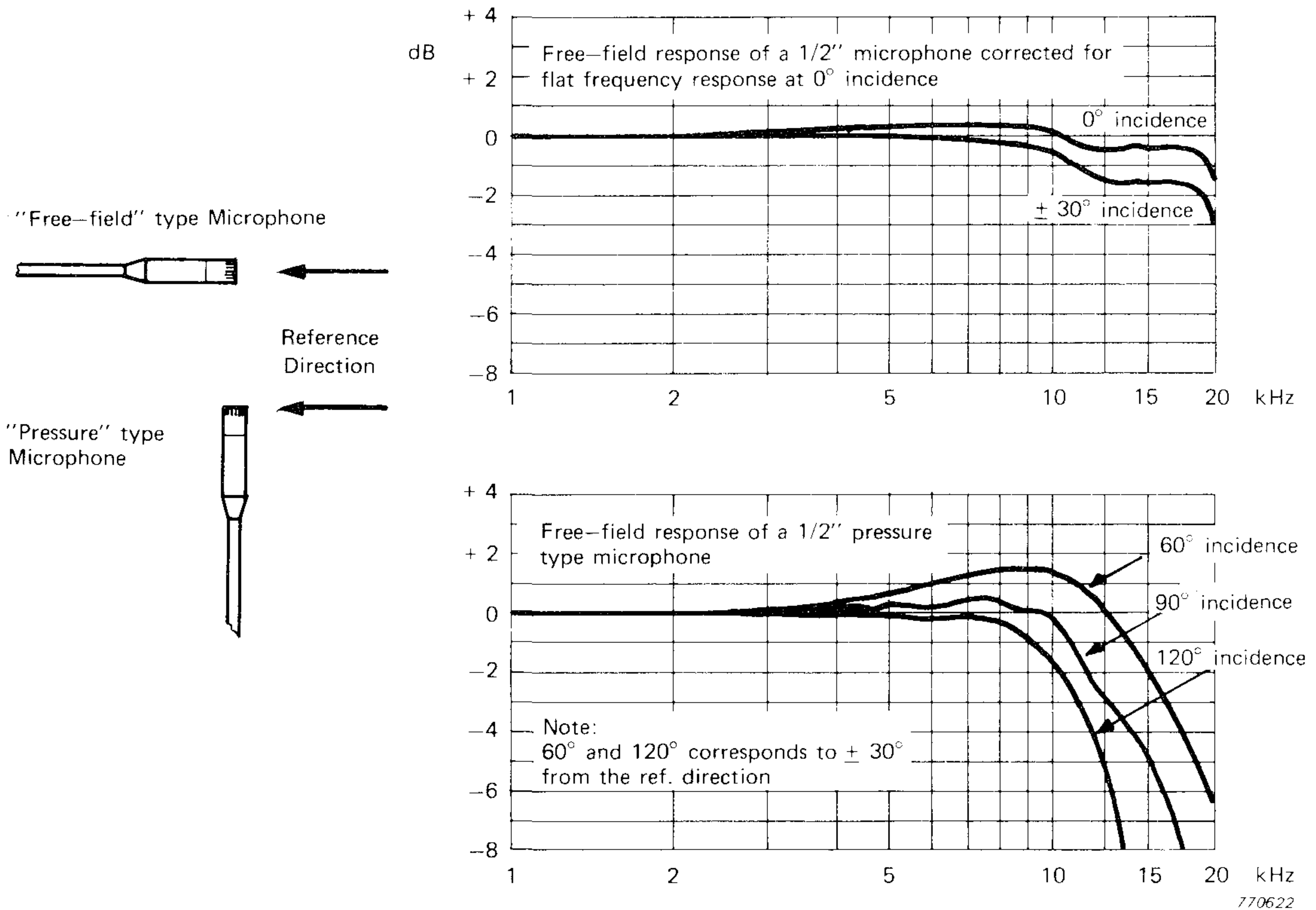
Fig.7. Comparison between the free-field frequency response of a "Free-field" and a "pressure" type microphone and their sensitivity deviations due to small changes in the angle of sound incidence from the reference direction
