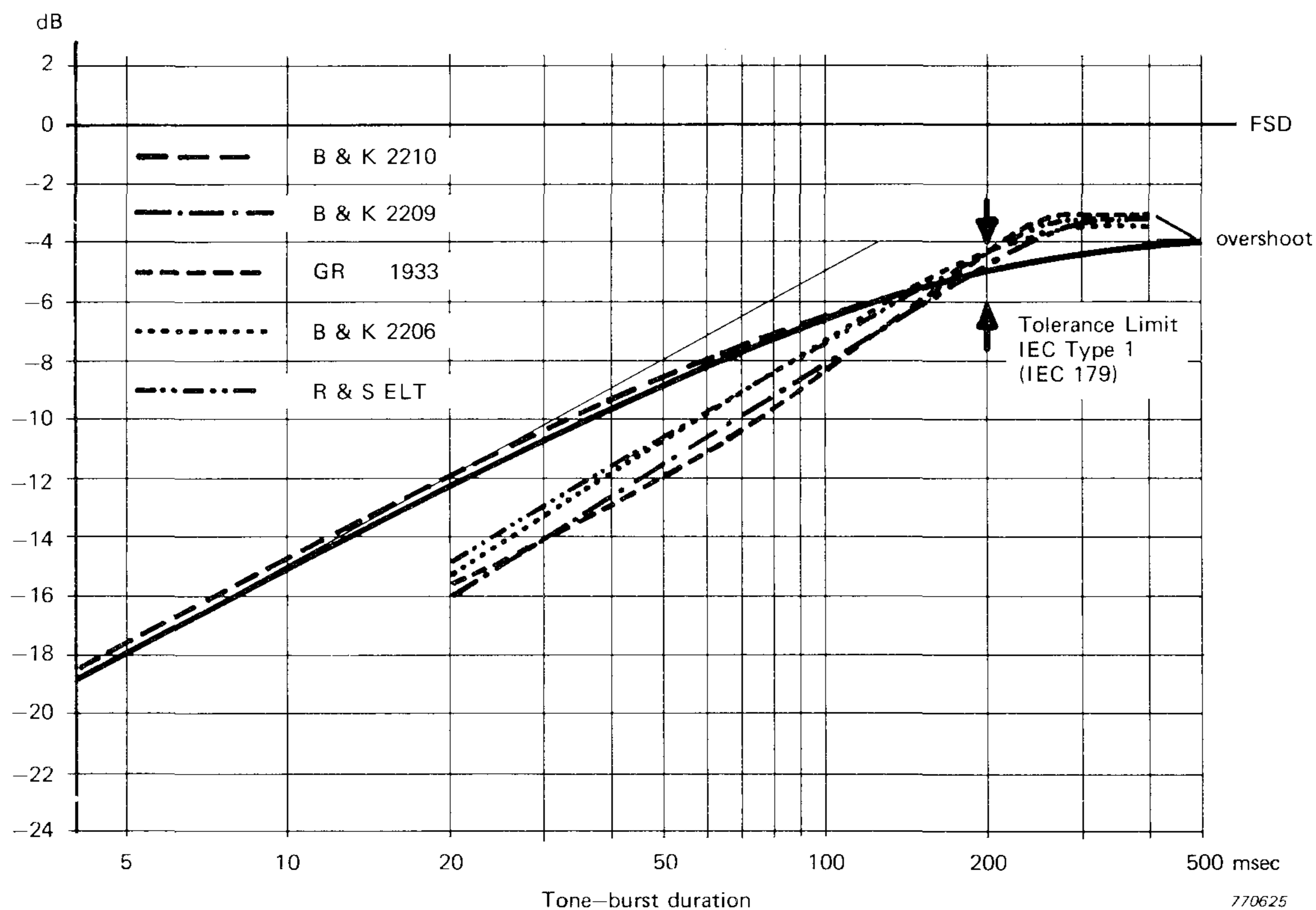
Fig.10. "Fast" response of different Sound Level Meters to a 2 kHz tone-burst. Reference is a continuous 2 kHz tone with the same amplitude as for the tone-burst. Reference level is 4 dB below FSD
